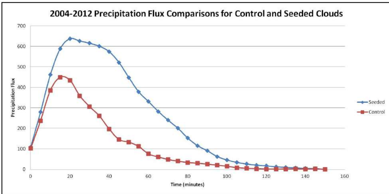
Figure 4: Precipitation flux (2004-2012) for seeded clouds versus control clouds (Ruiz-Columbiè et al., 2014). (kg/m²-s)
